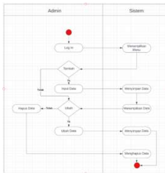
Gambar 3.2 Activity Diagram
