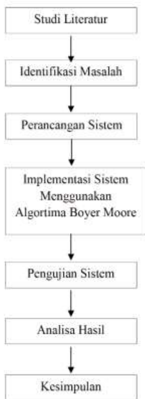
Gambar 3.1 Prosedur Penelitian
