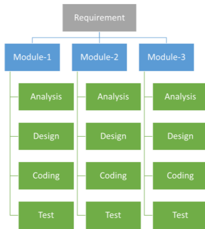
Gambar 2. Model incremental
