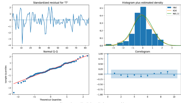
Gambar 7. Plot Diagnostik
