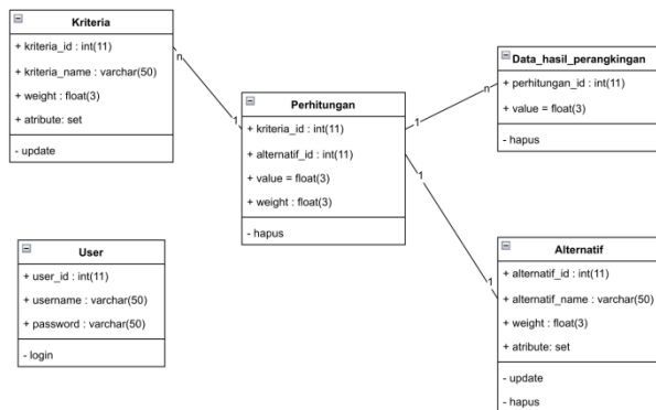
Gambar 5. Rancangan Class Diagram
