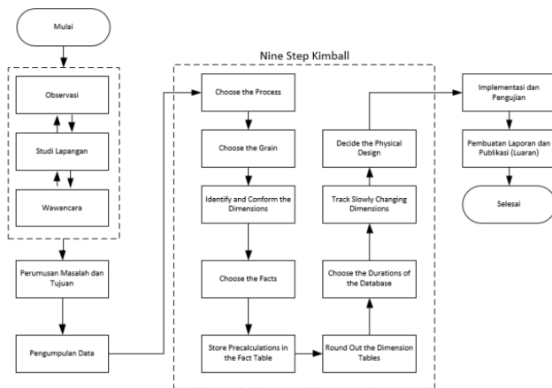
Gambar. 1 Metode Penelitian
