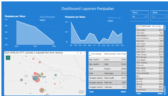
Gambar 6. Dashboard Laporan
