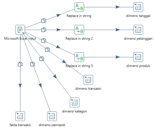
Gambar 4. Proses ETL
