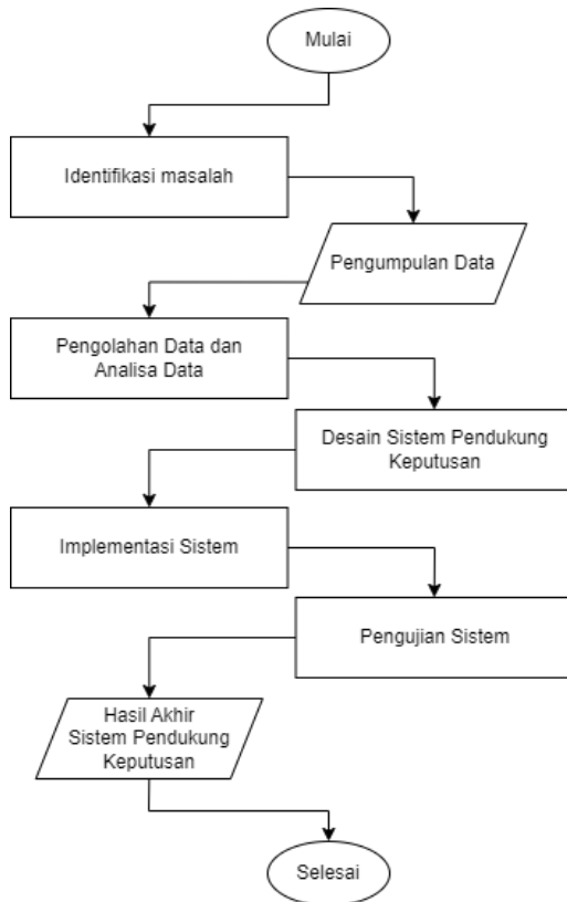
Gambar 1. Alur Penelitian
