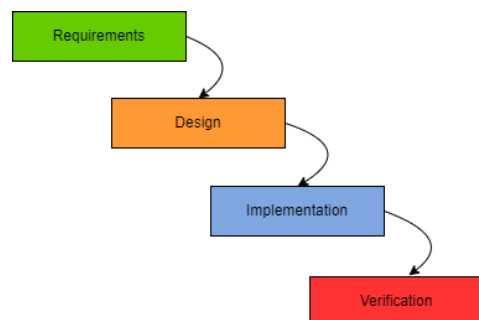
Gambar 2. Metode Waterfall
