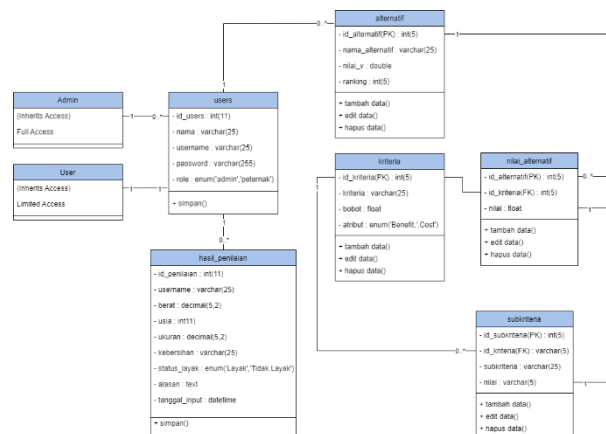
Gambar 4. Class Diagram
