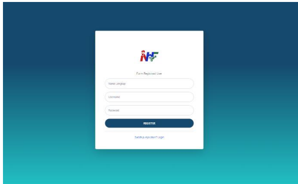
Gambar 5. Halaman Register
