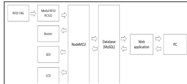
Gambar 2. Blok Diagram
